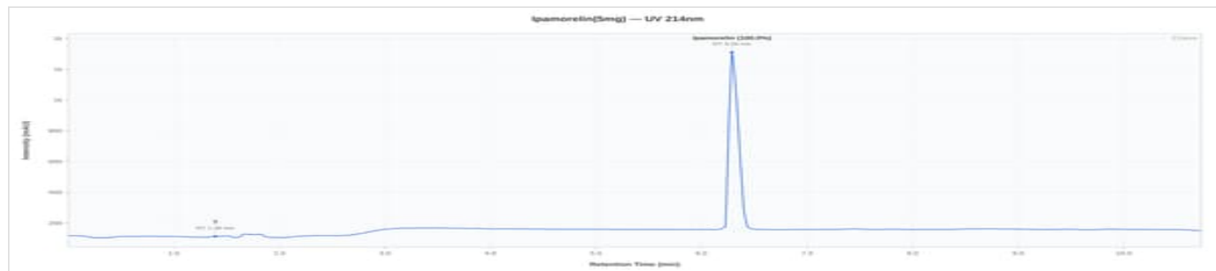
Ipamorelin 5mg - 2026060208: UV Chromatogram
